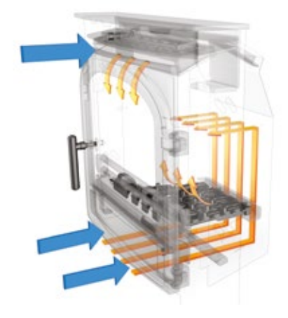
INSET AIRFLOW
