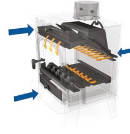
CONSORT AIRFLOW
